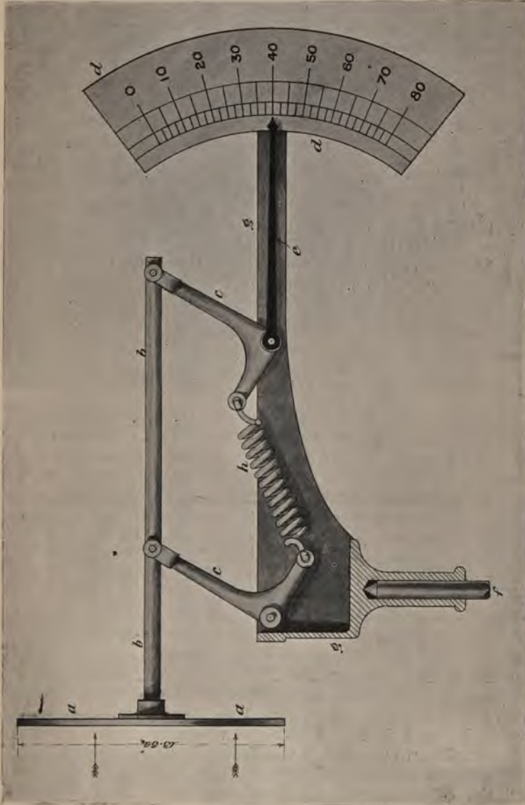
Fig. 38.—Apparatus for indicating the force and velocity of the wind direct without any timing, counting, or mathematical calculations.
